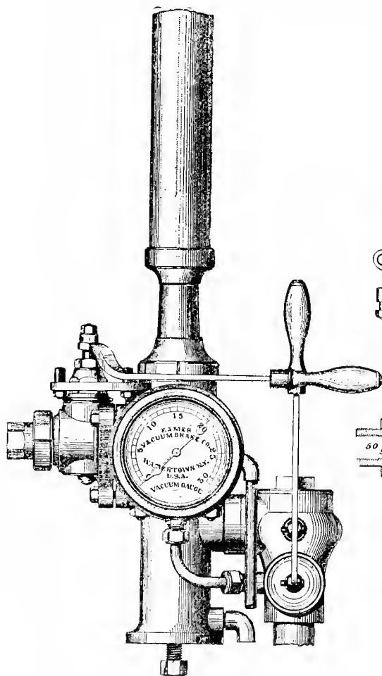
Fig. 1663. Elevation.
